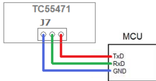
Figure 3-4 MCU to TC55471 Controller Connection
