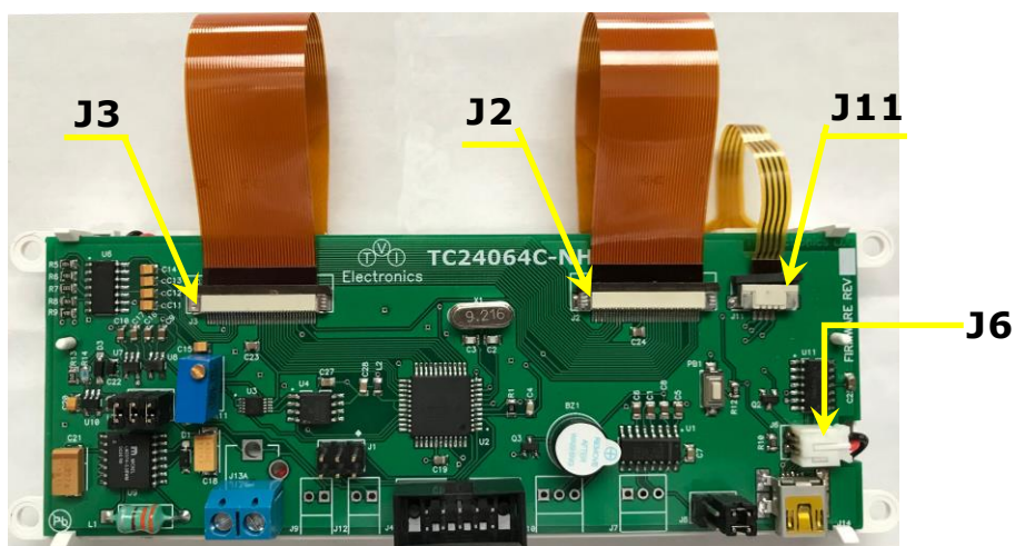
Figure 2-2: Hardware Connection
