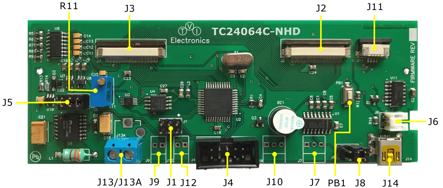
Figure 3-1: TC24064C-NHD Controller Board Layout
